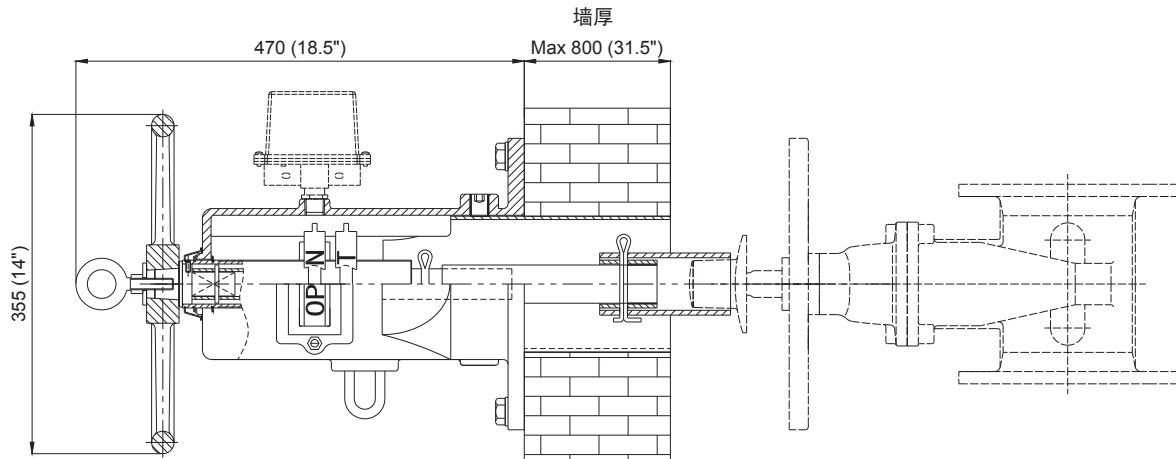
FIG. F0800-WP (4" ~ 14")
